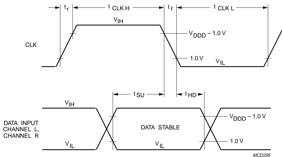
Fig.3 Timing waveform.
